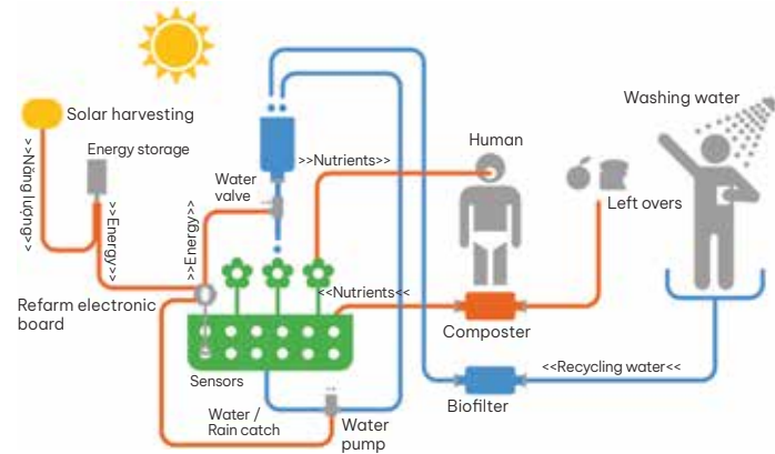
Figure 9.5b. Aquaponic gardening diagram (Source: www.gardeningsite.com)
