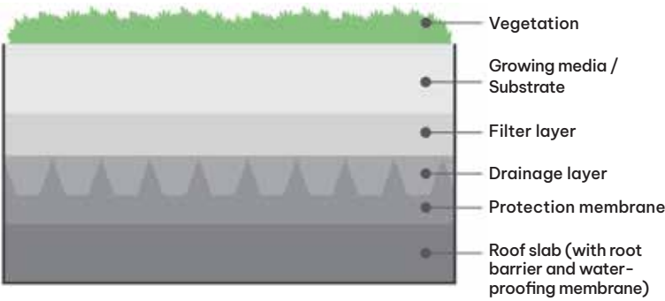
Figure 9.4a. Roof greening diagram (Source: Nguyen Quang Minh, 2022)
