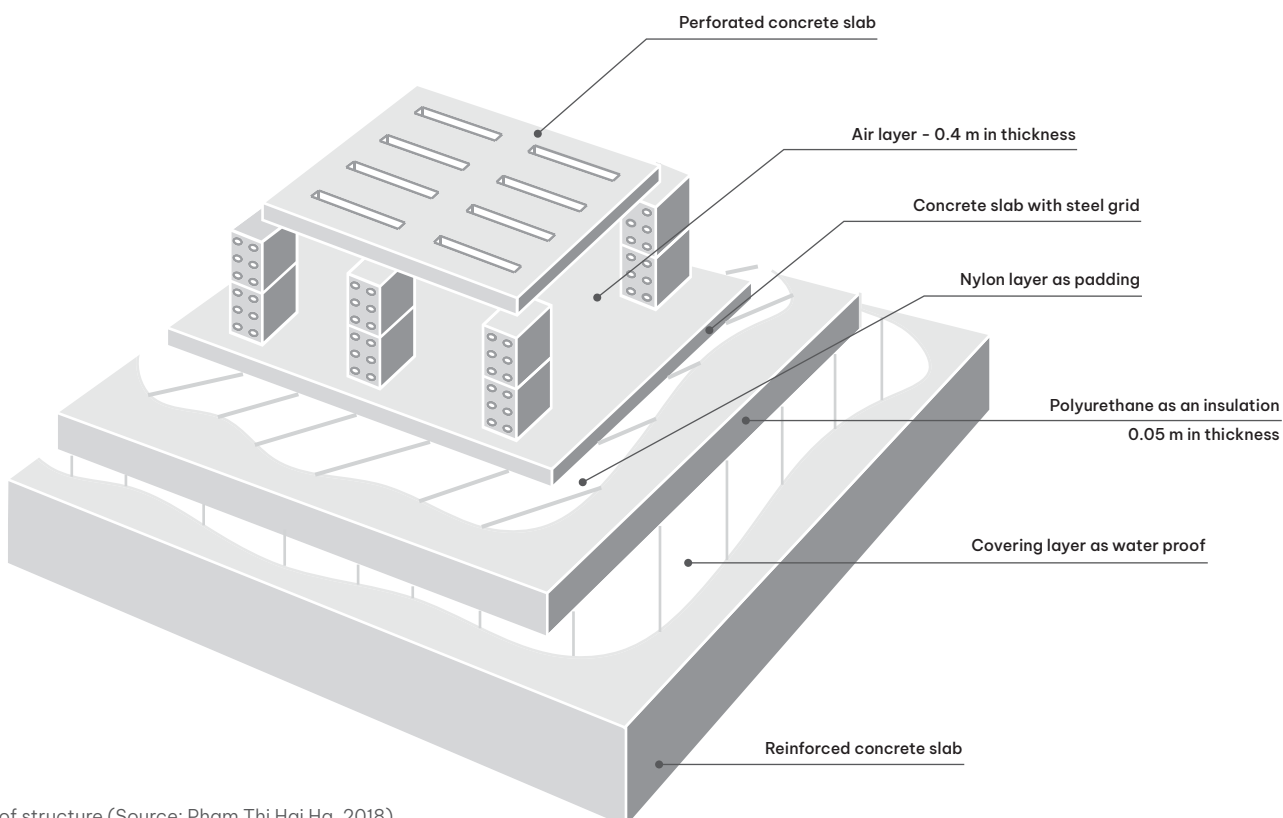
Figure 3.3c. Roof structure (Source: Pham Thi Hai Ha, 2018)
