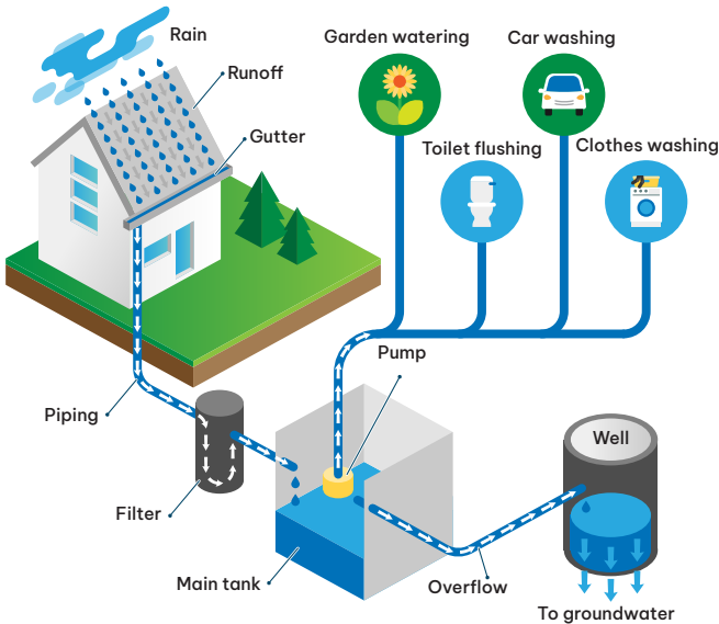
Figure 11.3b. Rainwater is collected for various purposes in place of tap water (Source: www.gutterhelmet.com)
