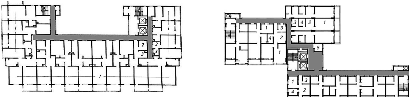
Figure 2.8. Floor plan of a 15-story building (1985) (picture left) and a 20-story building (1987) for reference (Source: Li Zhenyu, 2009)
