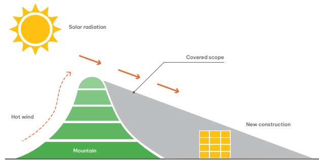
Figure 1.9a. Reducing heat by making full use of shade from a nearby hill (Source: Nguyen Quang Minh, 2014)
