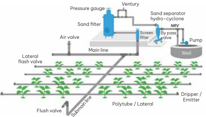
Figure 9.5a. Drip irrigation diagram (Source: www.gardeningsite.com)
