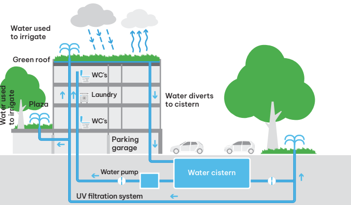
Figure 9.5e. Rainwater harvesting diagram (Source: www.studiohillier.com )
