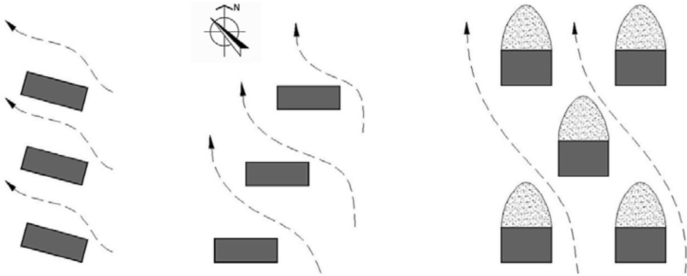
Figure 2.1. Solution for master planning of the housing area, enabling natural ventilation (Source: Ngo Le Minh, 2013)
